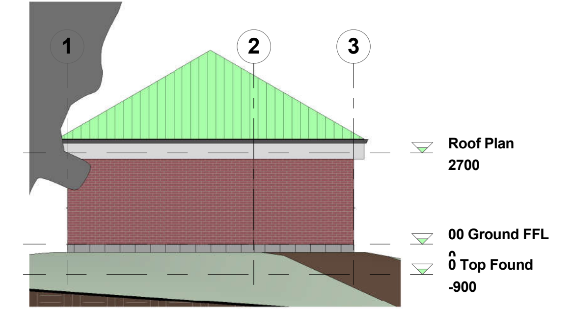
WEST ELEVATION 1 : 100
