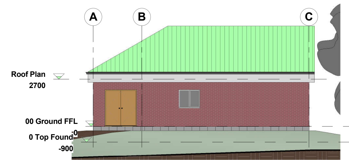
SOUTH ELEVATION 1 : 100
