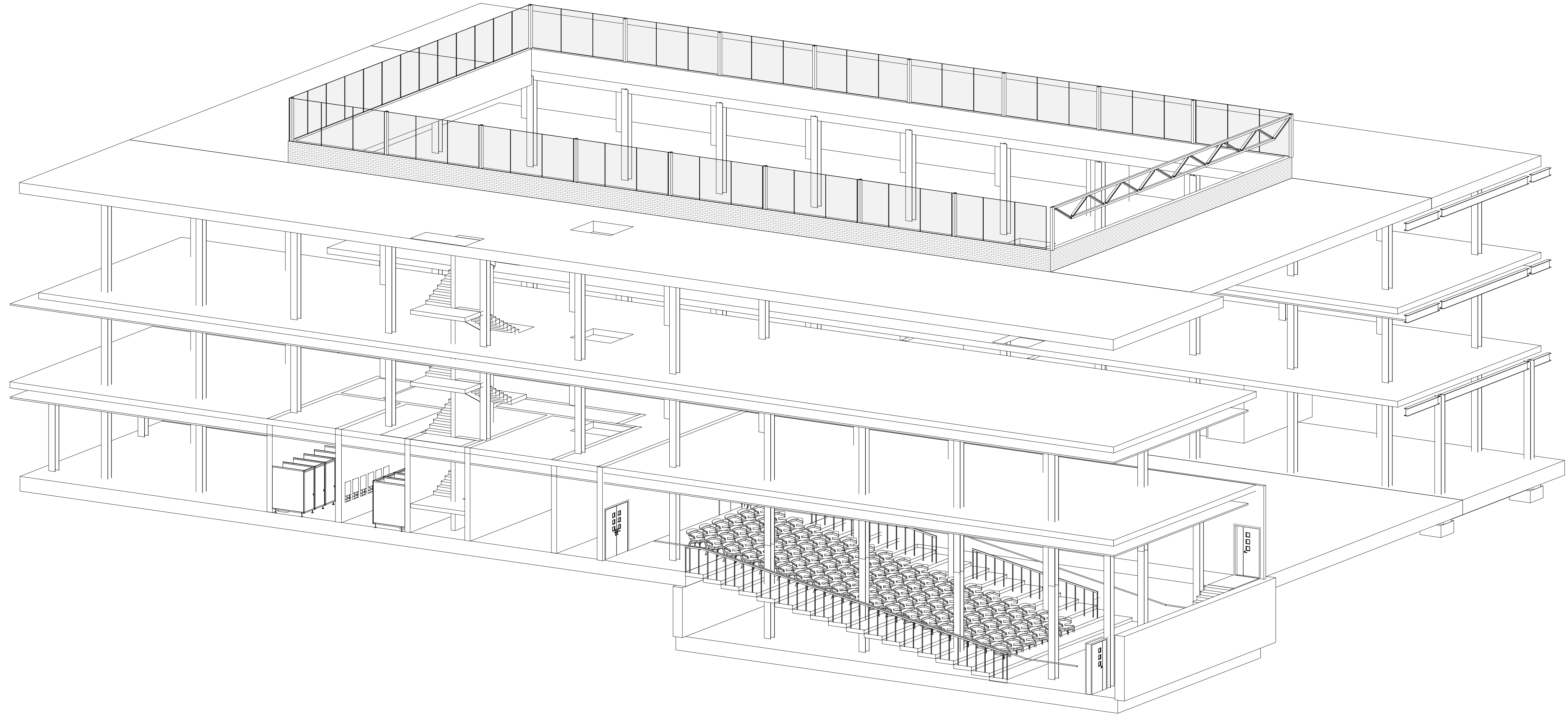
1 3D - Structural 3D View
